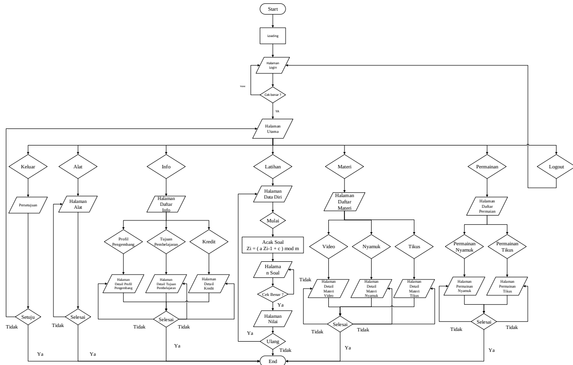
Gambar 2. Flowchart Sistem
