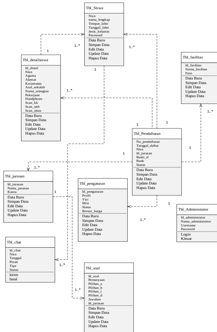
Gambar 4. Class Diagram
