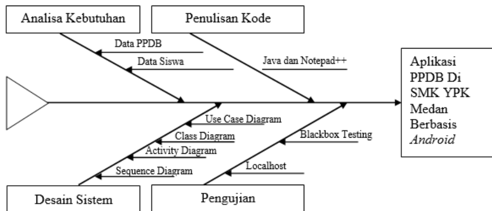
Gambar 1. Waterfall Diagram
