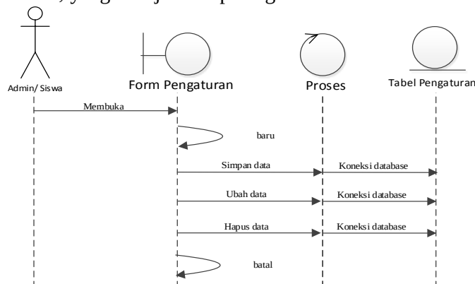
Gambar 11. Sequence Diagram Pengaturan
