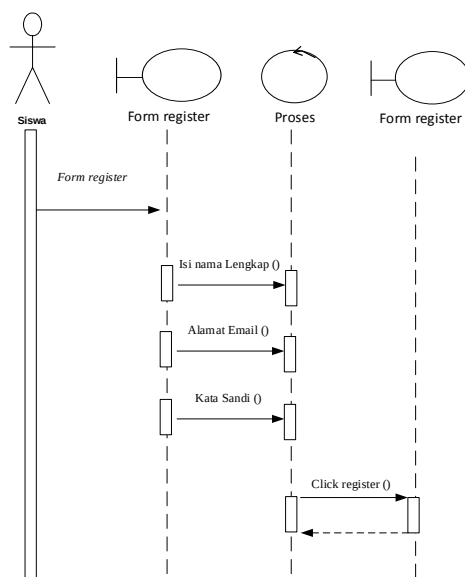
Gambar 10. Sequence Diagram Register
