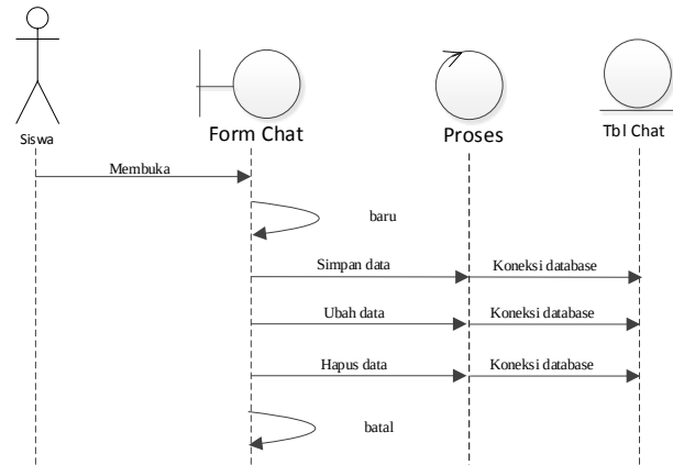
Gambar 16. Sequence Diagram Chat
