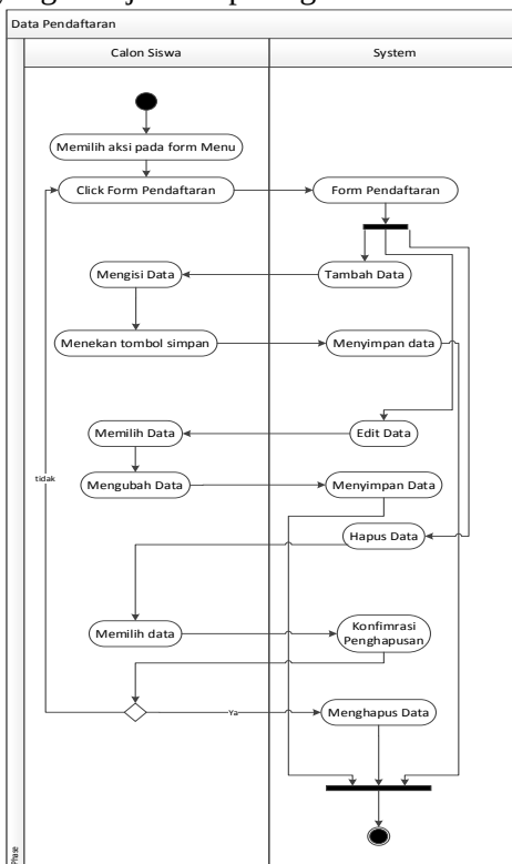
Gambar 7. Activity Diagram Pendaftaran
