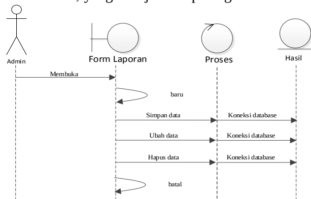
Gambar 19. Sequence Diagram Laporan Diterima
