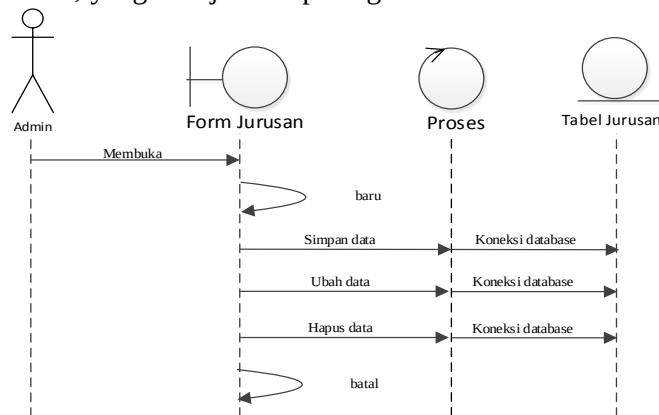
Gambar 13. Sequence Diagram Jurusan
