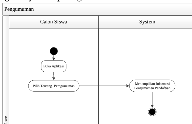
Gambar 8. Activity Diagram Pengumuman
