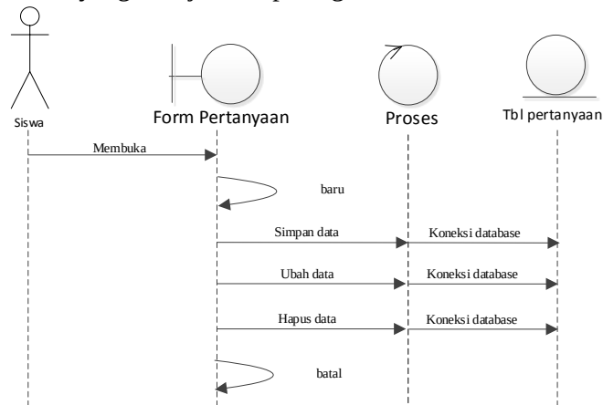
Gambar 15 Sequence Diagram Pertanyaan
