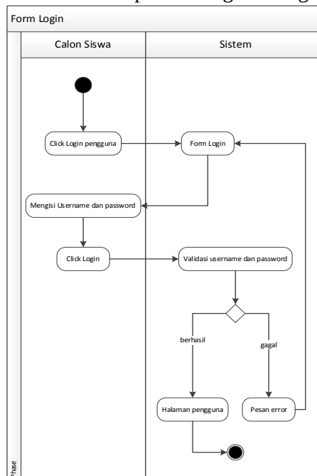
Gambar 6. Activity Diagram Login
