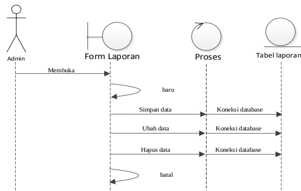
Gambar 18. Sequence Diagram Laporan Sisswa Ditolak
