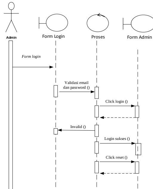
Gambar 9. Sequence Diagram Login
