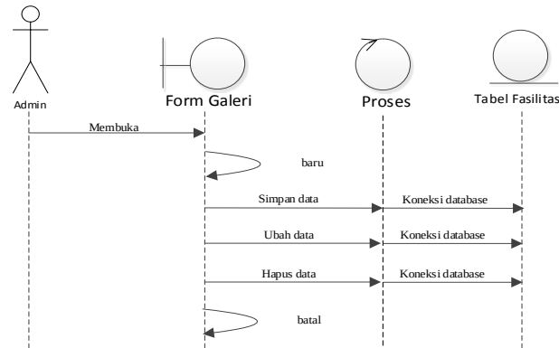
Gambar 12. Sequence Diagram Galeri
