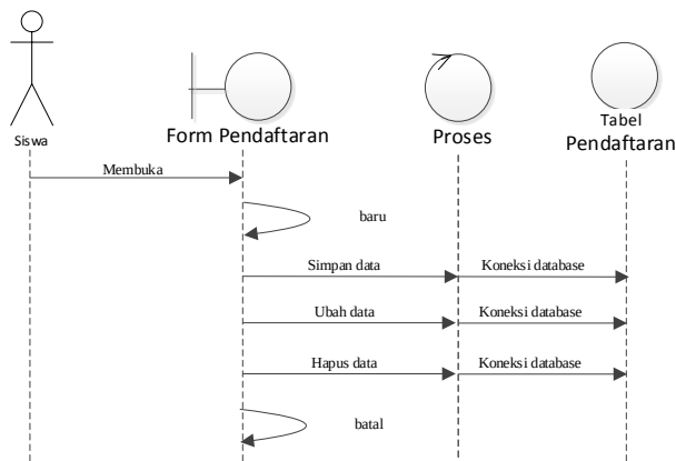
Gambar 14. Sequence Diagram Pendaftaran
